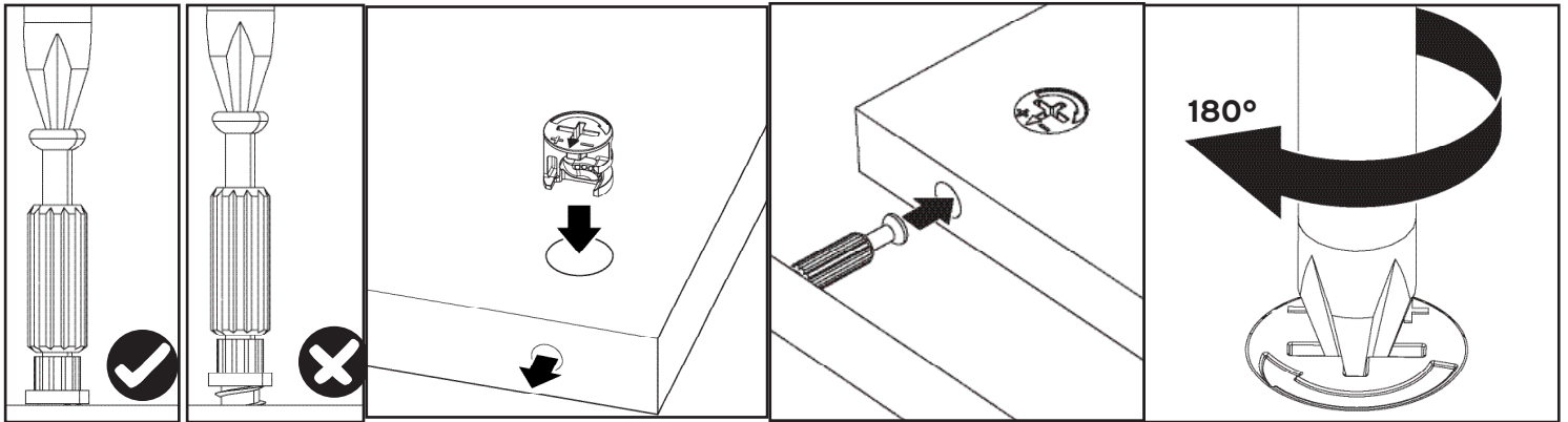
Electric Screwdriver + Torque set at 3-5
